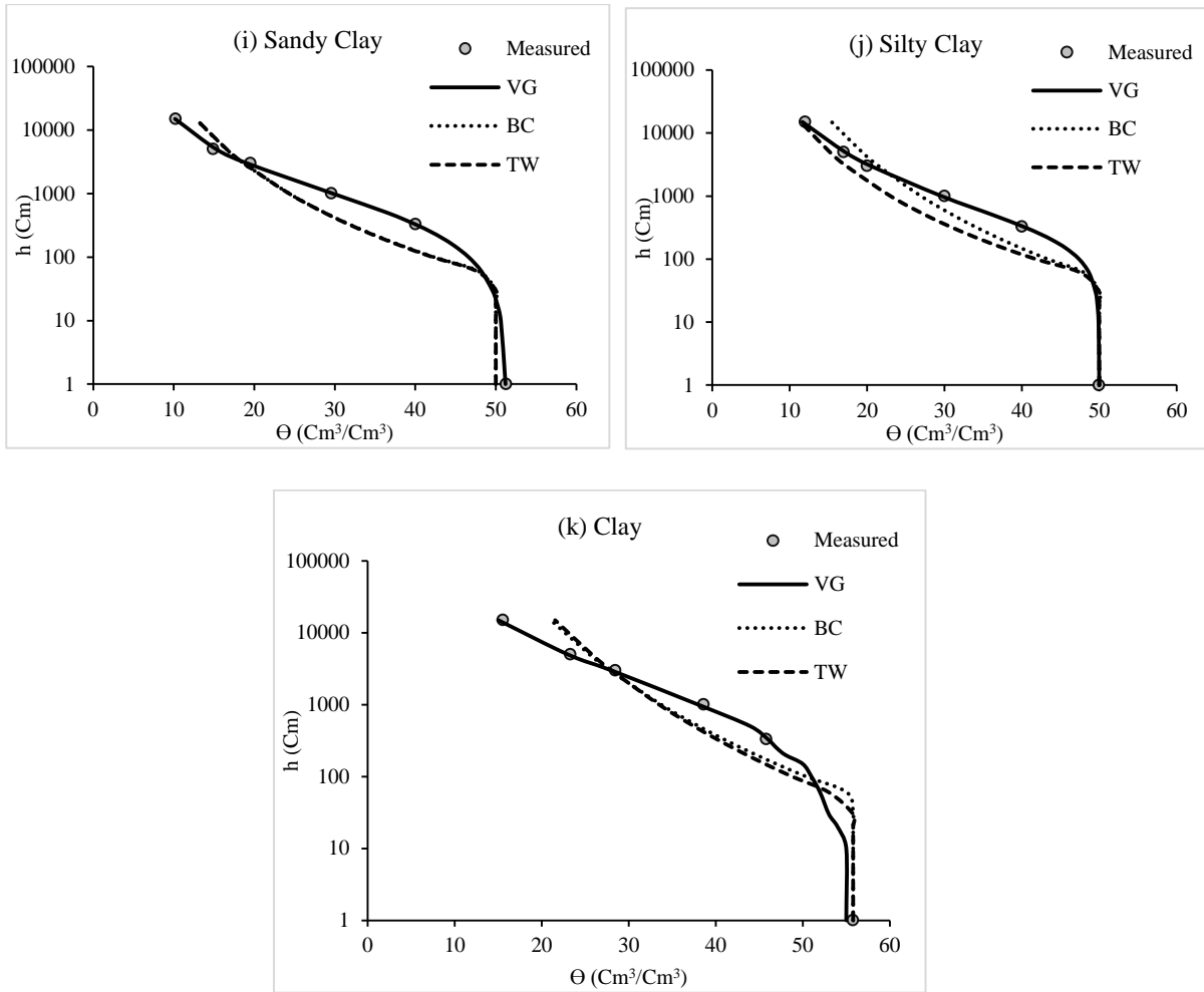
Fig. 2. The measured and predicted retention curves by different models for different soil textures.
