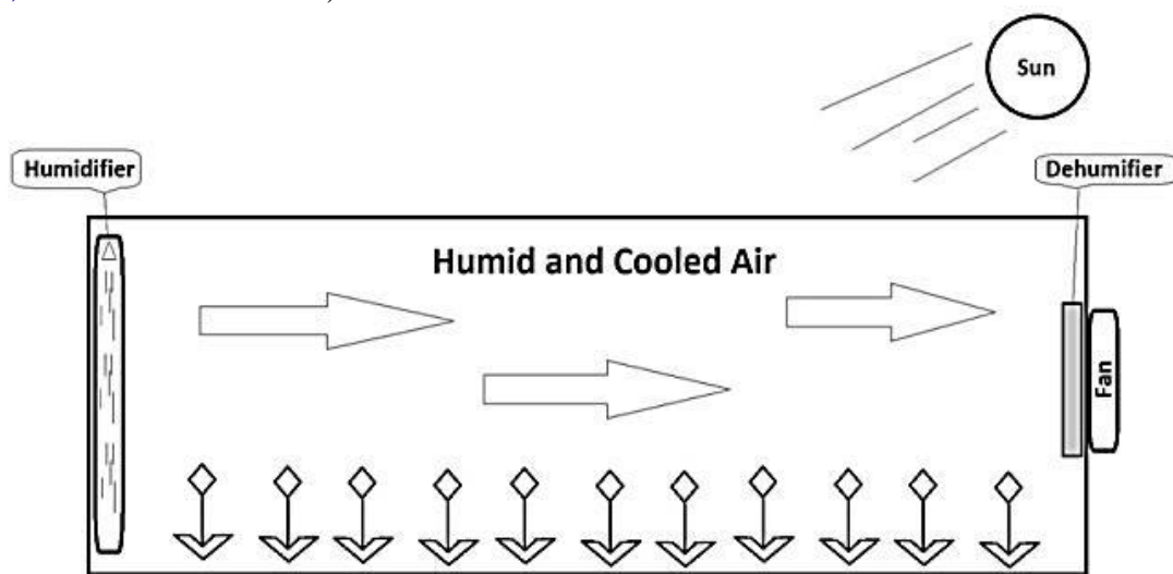
Fig. 1. Seawater Greenhouse
